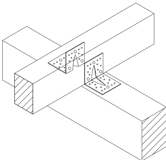
Typical installation
